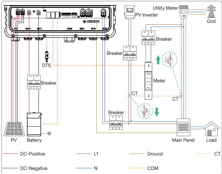
AC Coupled System
